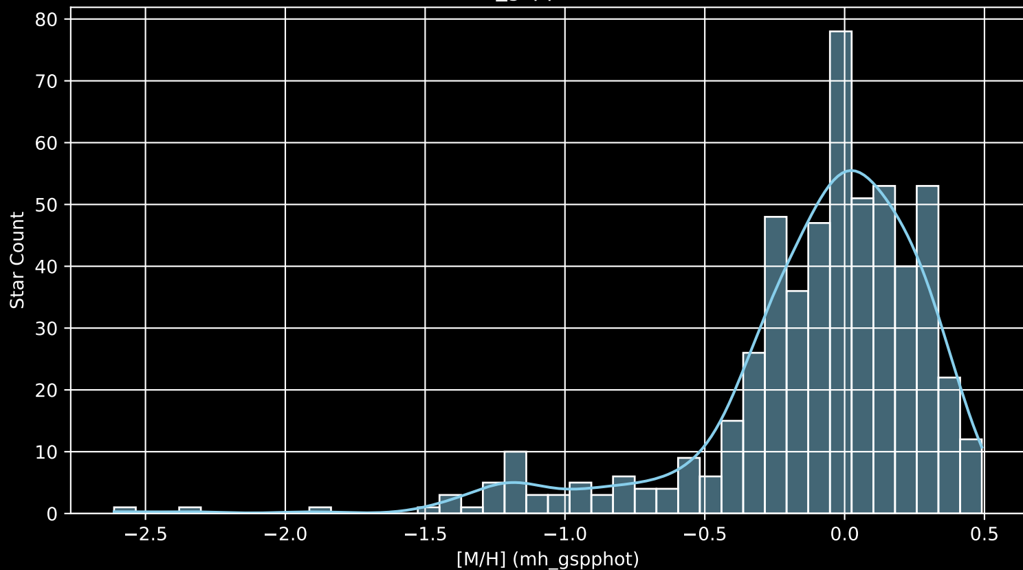
APOGEE DR17 Field: [020+04 [M/H] (mh_gspphot) (n= 547)
