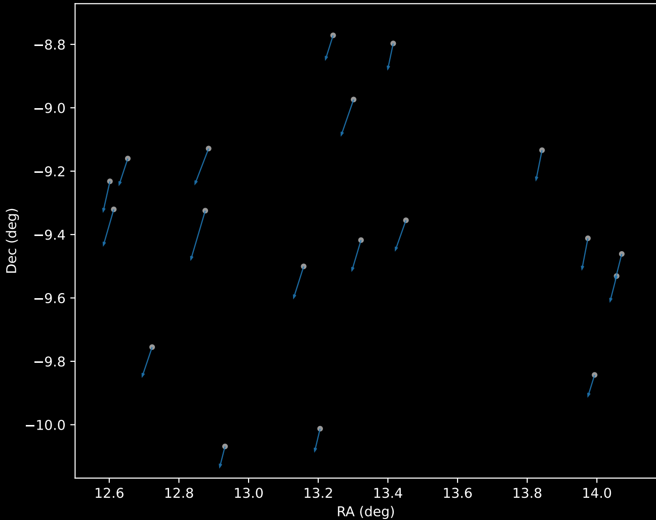
APOGEE DR17 Cluster 20 Proper Motion Vectors (n=19)
