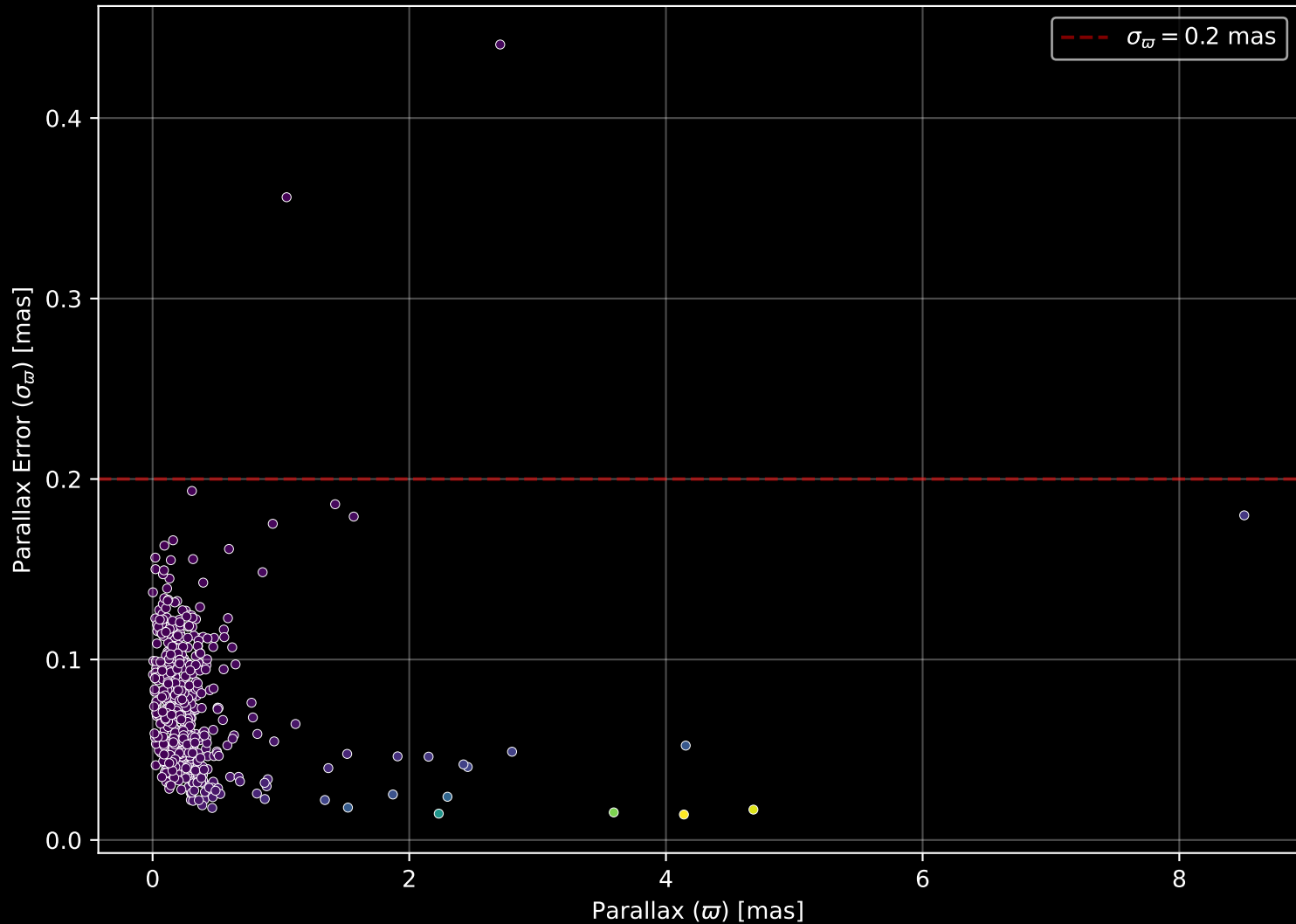
APOGEE DR17 Field: [020+04] Parallax Quality (n= 564)
