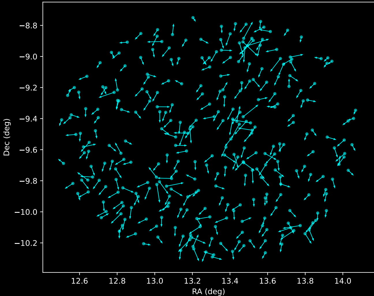
APOGEE DR17 Noise Stream Proper Motion Vectors (n=306)
