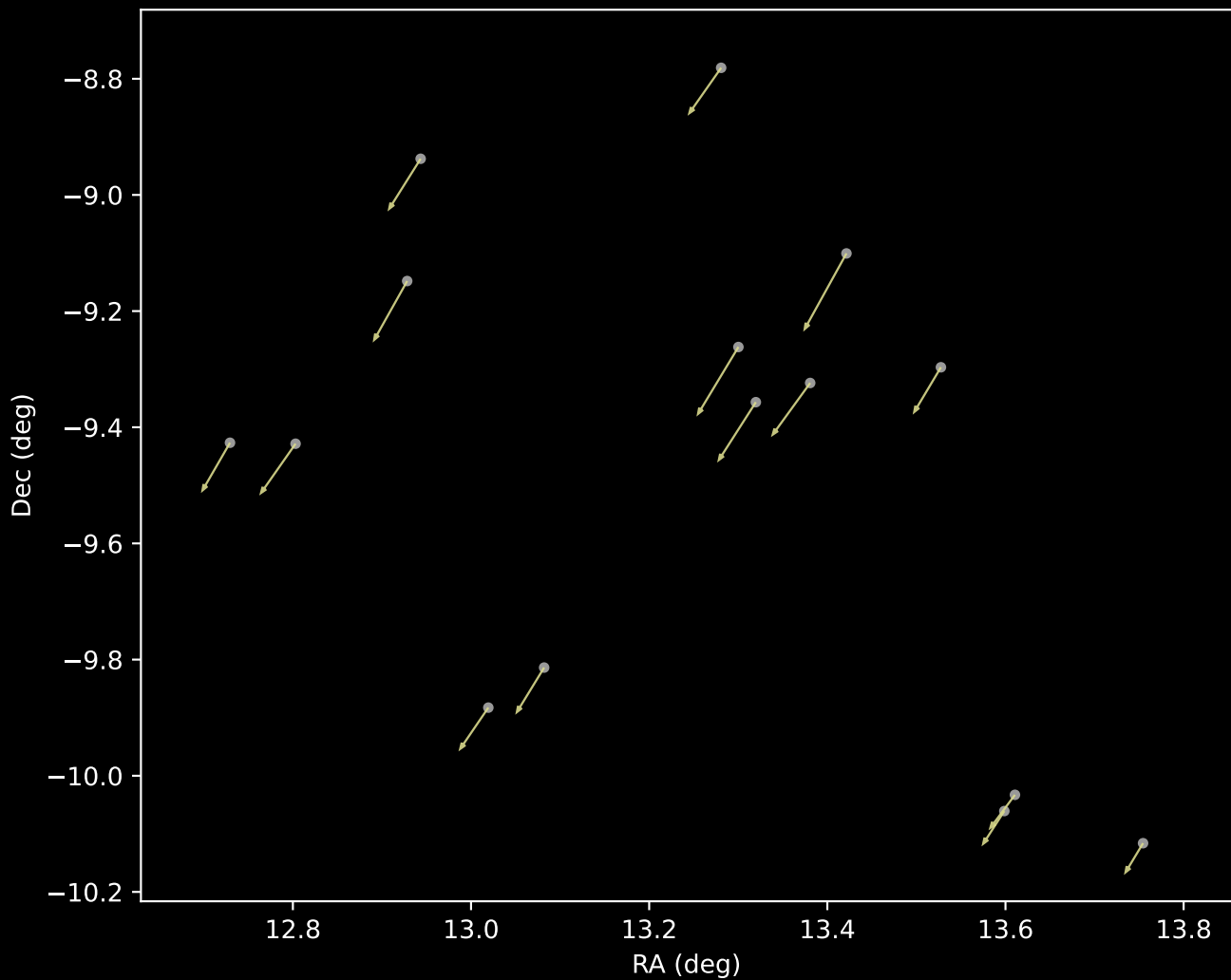
APOGEE DR17 Cluster 17 Proper Motion Vectors (n=15)
