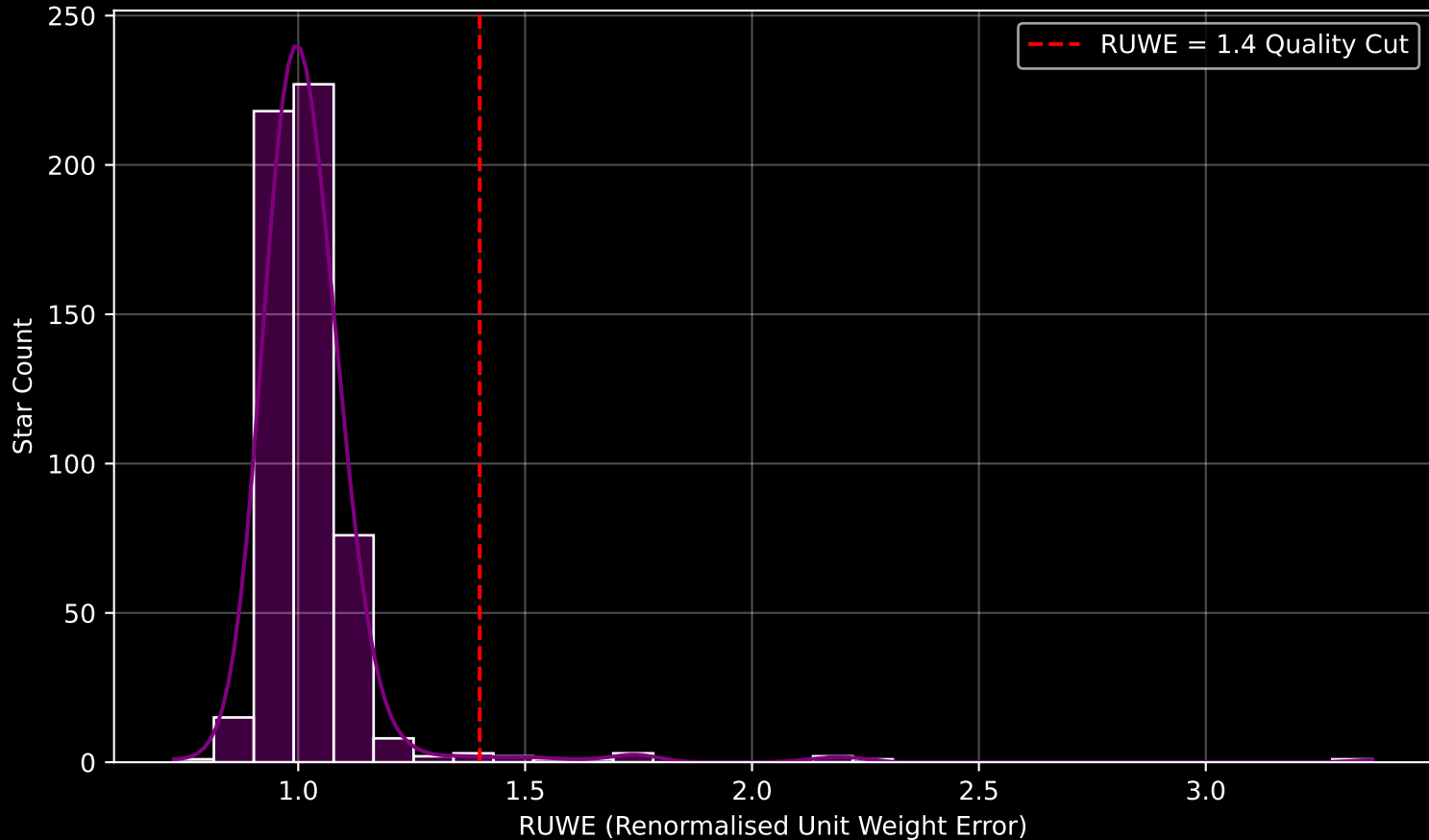
GAPOGEE DR17 Field [020+04] RUWE Distribution (n= 561)
