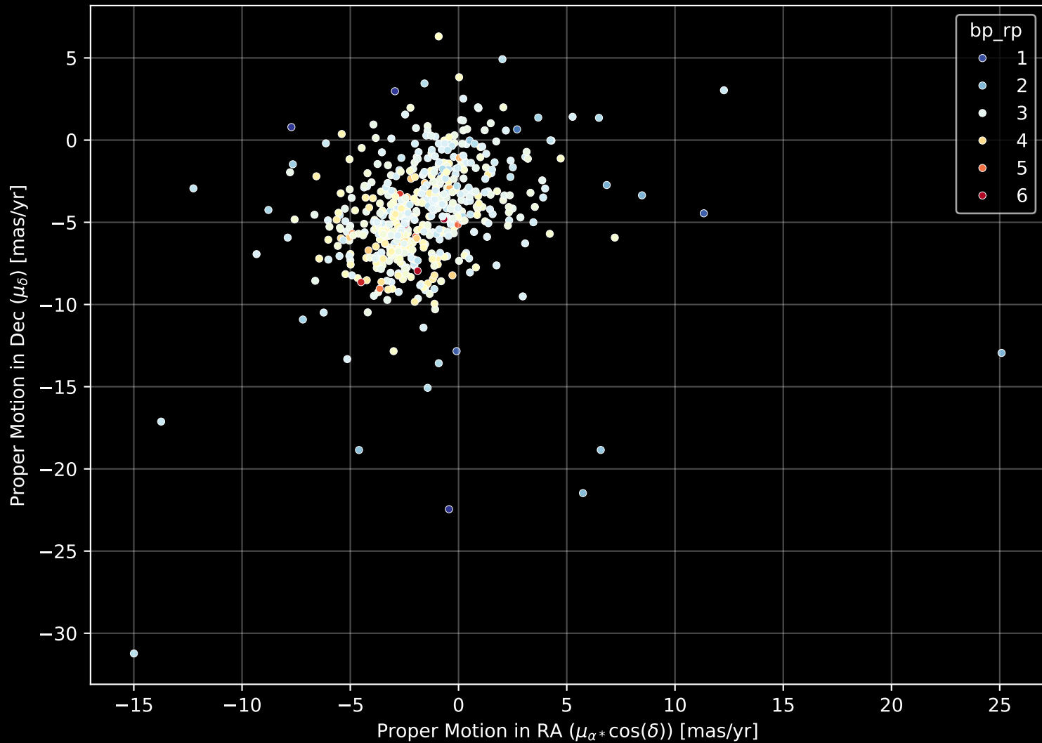
APOGEE DR17 Field: [020+04] Proper Motion Diagram (n= 564)
