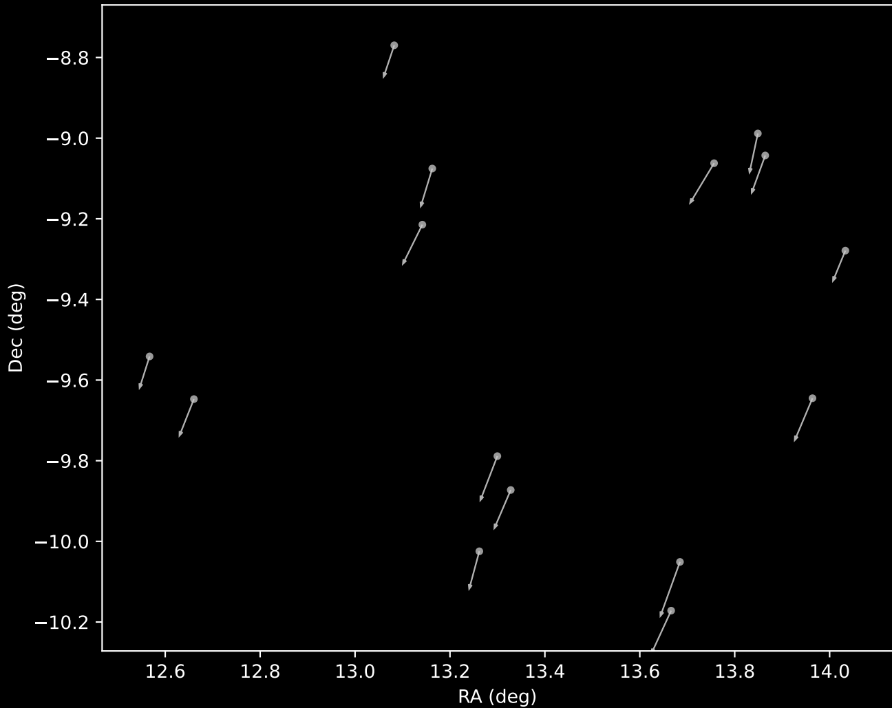
APOGEE DR17 Cluster 15 Proper Motion Vectors (n=15)
