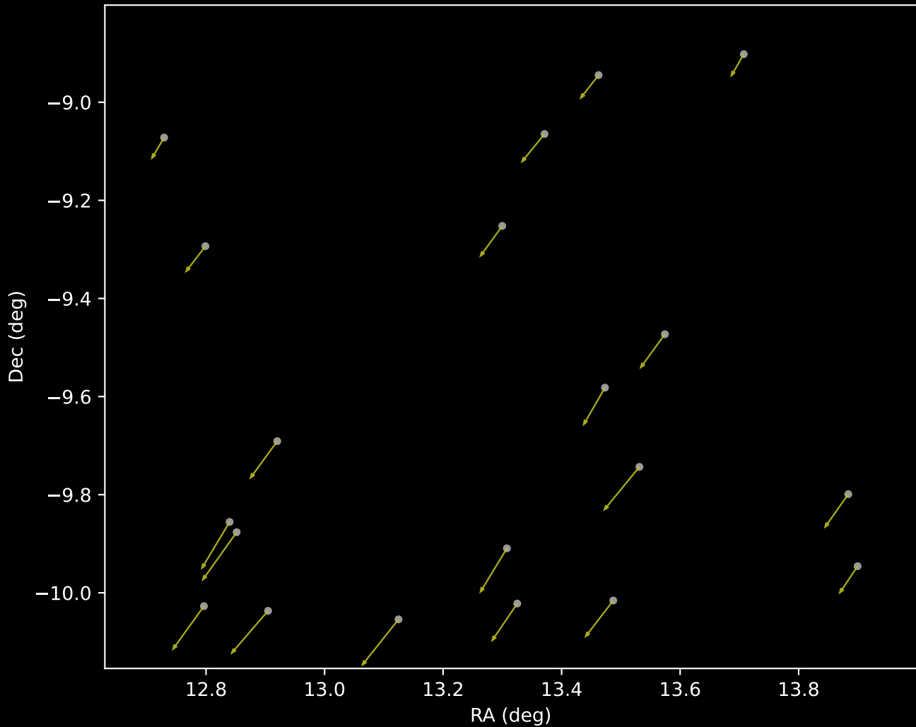
APOGEE DR17 Cluster 16 Proper Motion Vectors (n=20)
